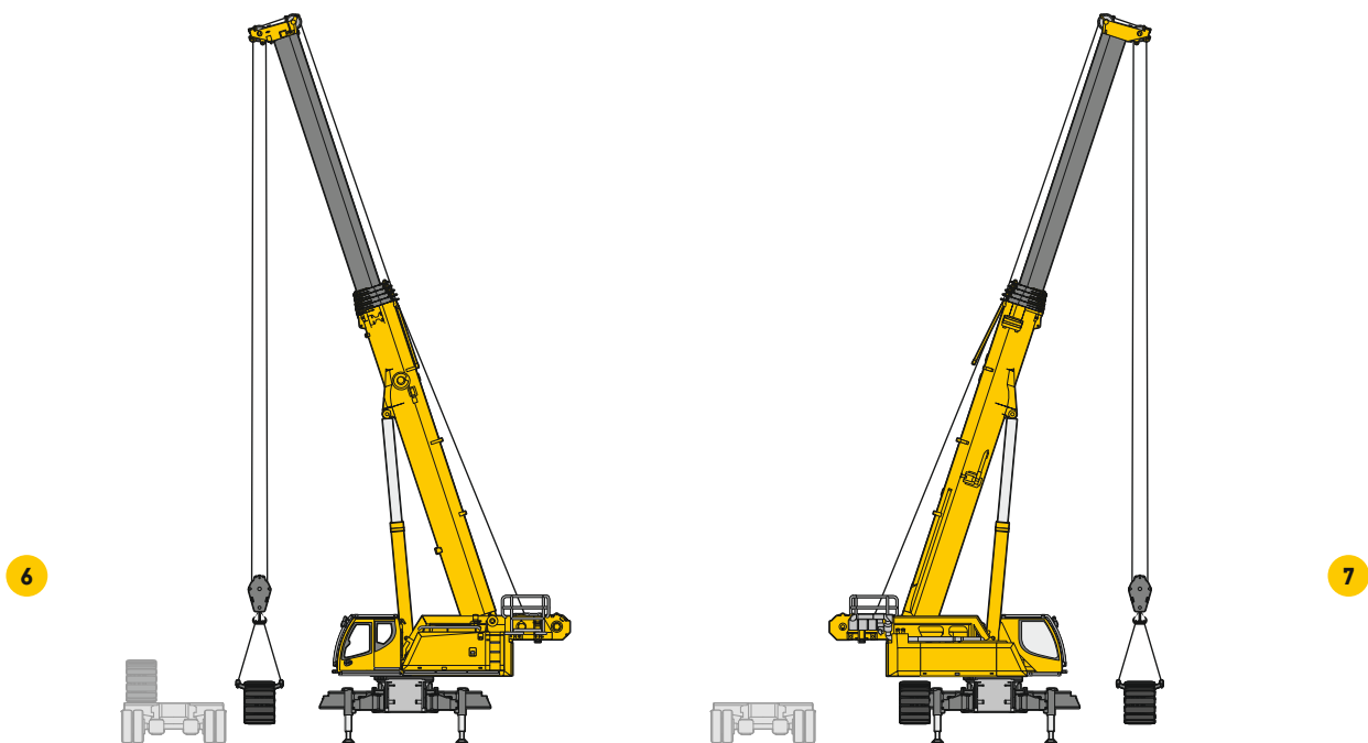
Extend the crawler tracks / Assemble the crawler tracks Sortir les supports transversaux / montage des chenilles
