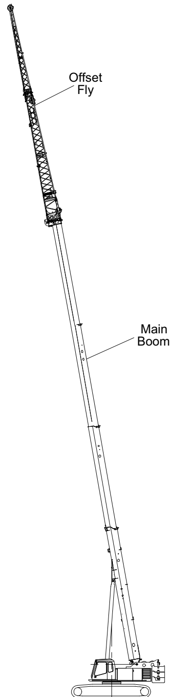
38.6-120.1 ft (11.8-36.6m) Main Boom With 35-58 ft (10.7-17.7m) Offset Fly
